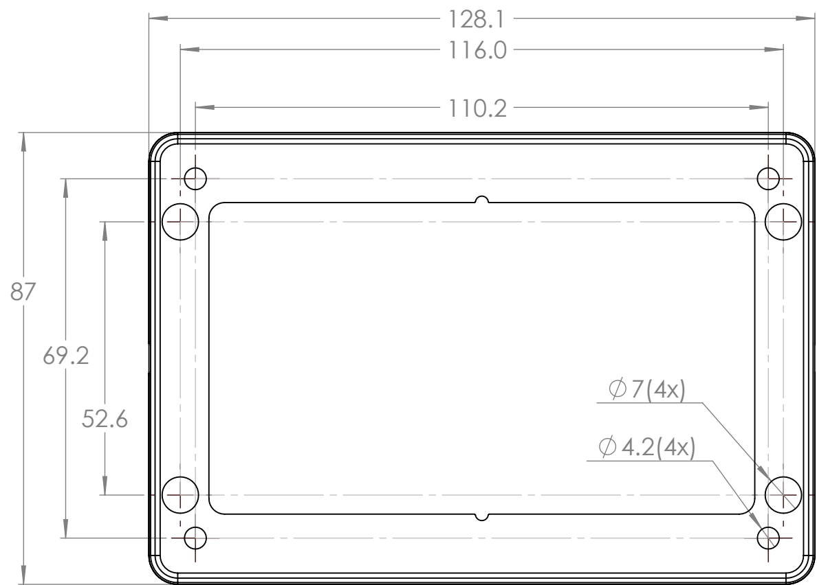
Frame dimensions
