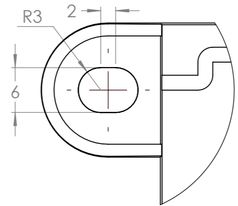
DETAIL A 2x SCALE 2:1
