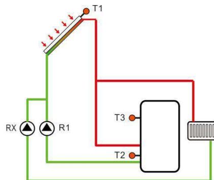
Heat transfer by collector pump logic
